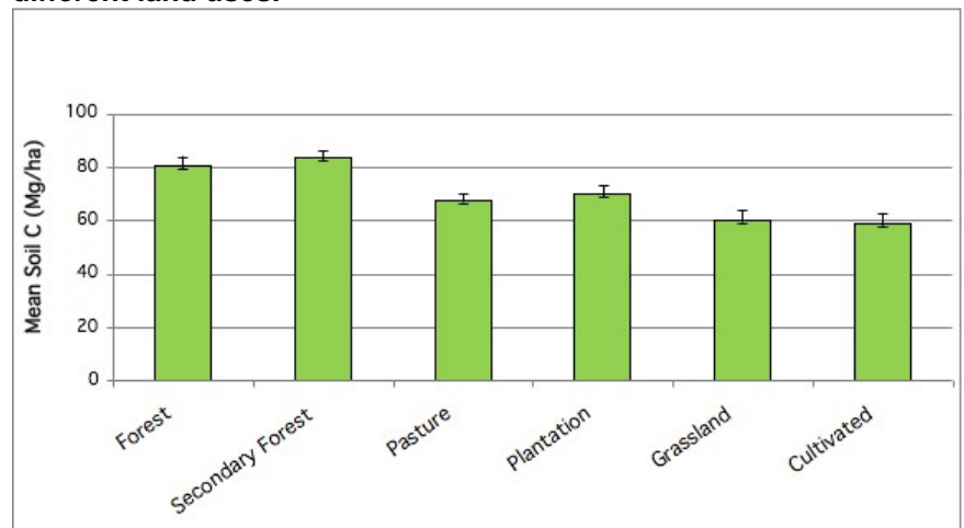
Figure 2. Comparison of mean soil carbon stocks to 30 cm under different land uses.
