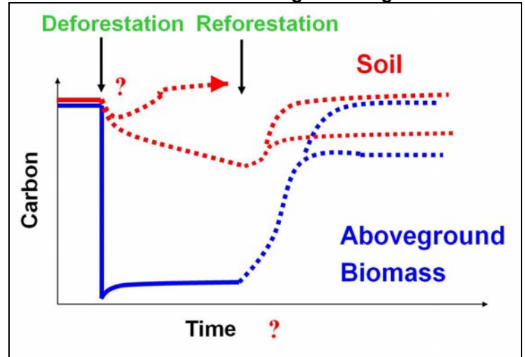
Figure 3. The impact of deforestation and reforestation on soil carbon vs. carbon in above ground vegetation.
